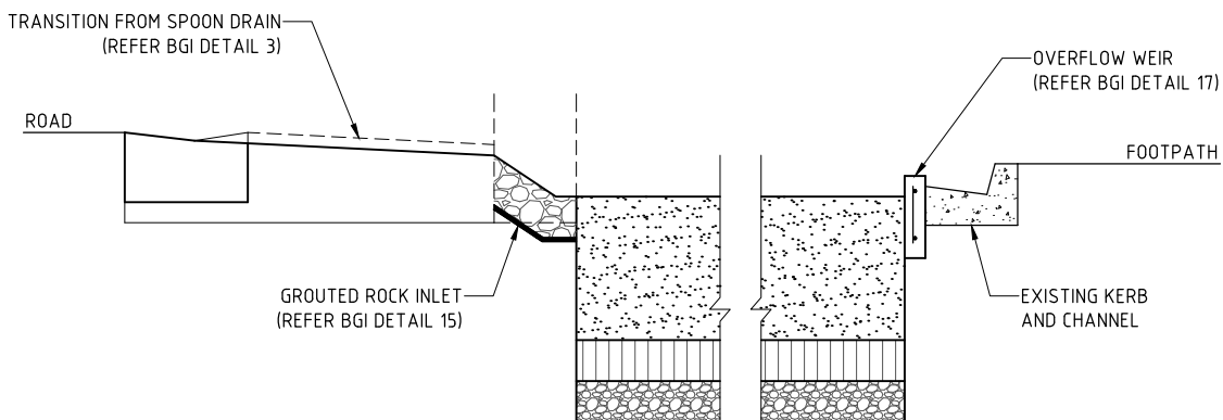
SECTION B-B
