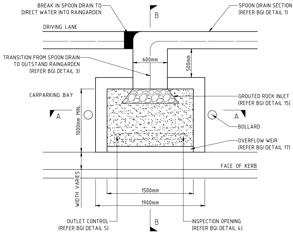
LAYOUT PLAN
