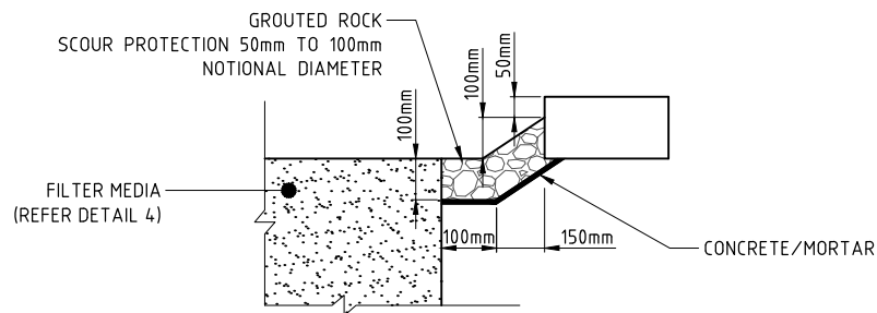
TYPICAL SECTION SCALE 1 : 20 @ A4
