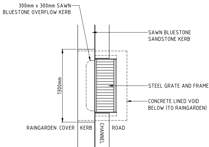
LAYOUT PLAN
