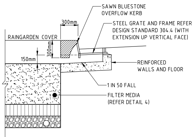
TYPICAL SECTION
