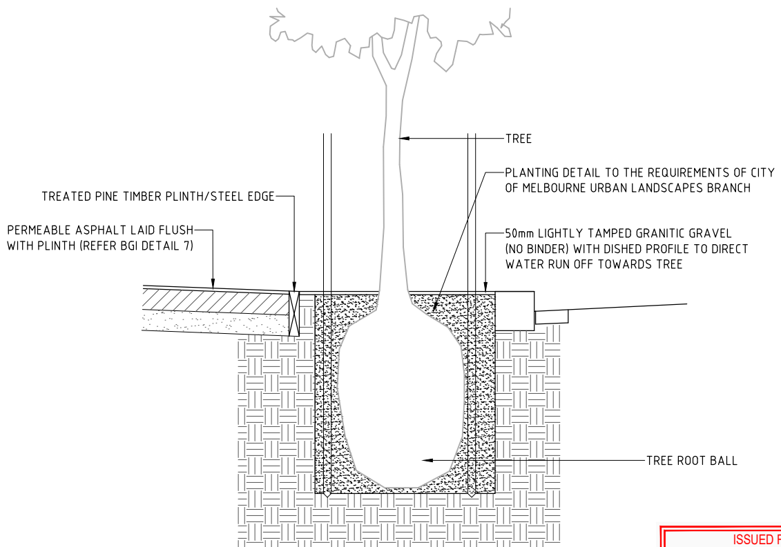
TYPICAL SECTION
