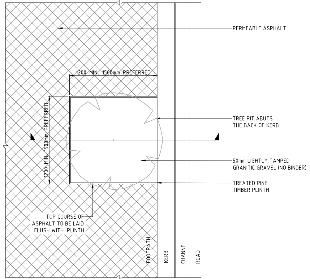
LAYOUT PLAN
