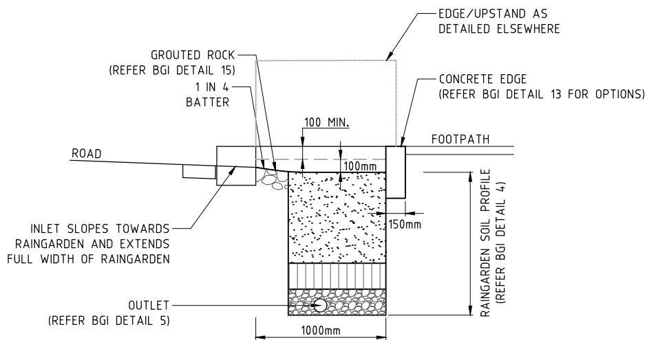
TYPICAL SECTION
