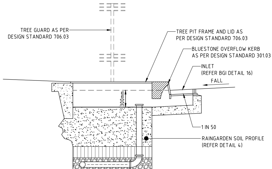
TYPICAL SECTION
