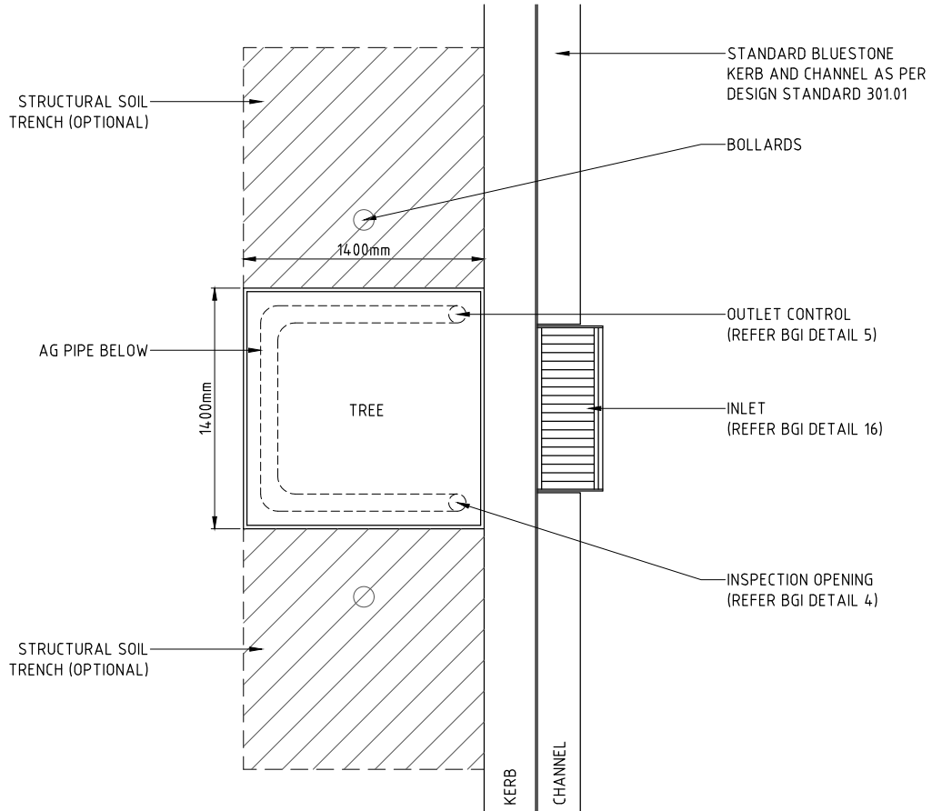
LAYOUT PLAN
