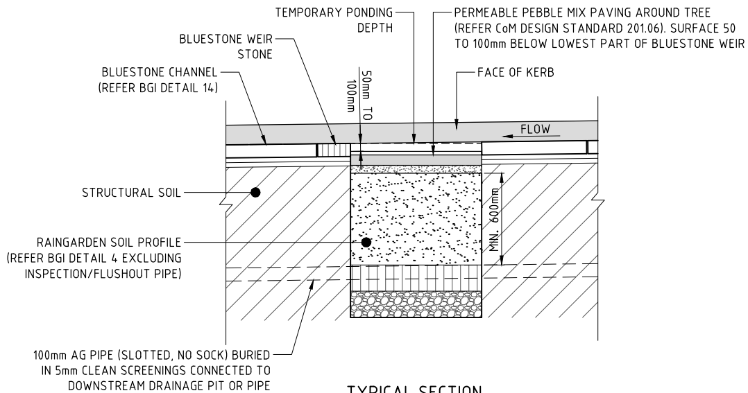
TYPICAL SECTION
