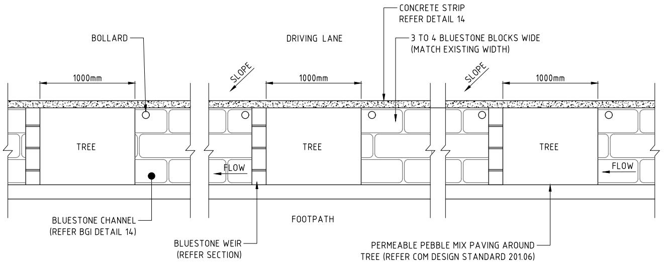
LAYOUT PLAN
